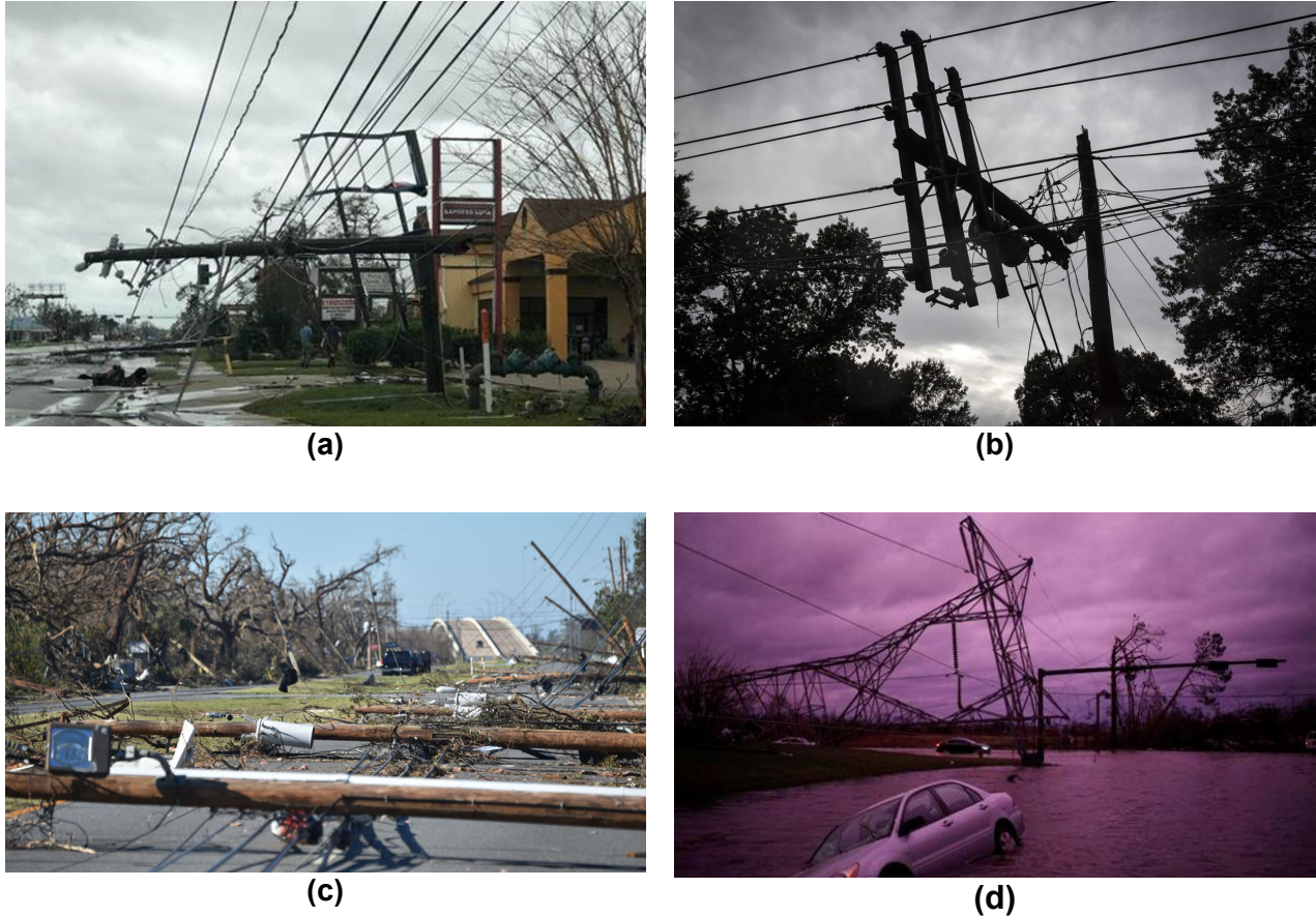
Figure 20: (a) Failed wooden power poles in Mexico Beach. (Source: Tallahassee Democrat); (b) Downed power lines in Winston-Salem, NC (Source: Winston-Salem Journal); (c) Fallen electrical poles block a road in the aftermath of Hurricane Michael on Oct. 12, 2018 in Panama City, FL representing a cascade failure in multiple poles that could be initiated either by fallen trees, extreme wind effects, or both (Source: Hector Retamal/AFP/Getty Images); (d) Vehicle sits partially submerged in floodwaters as a fallen electricity transmission tower lays on the ground in the background after Hurricane Michael hit in Panama City, FL on Wednesday, Oct. 10, 2018. (Source: Luke Sharrett/Bloomberg).
