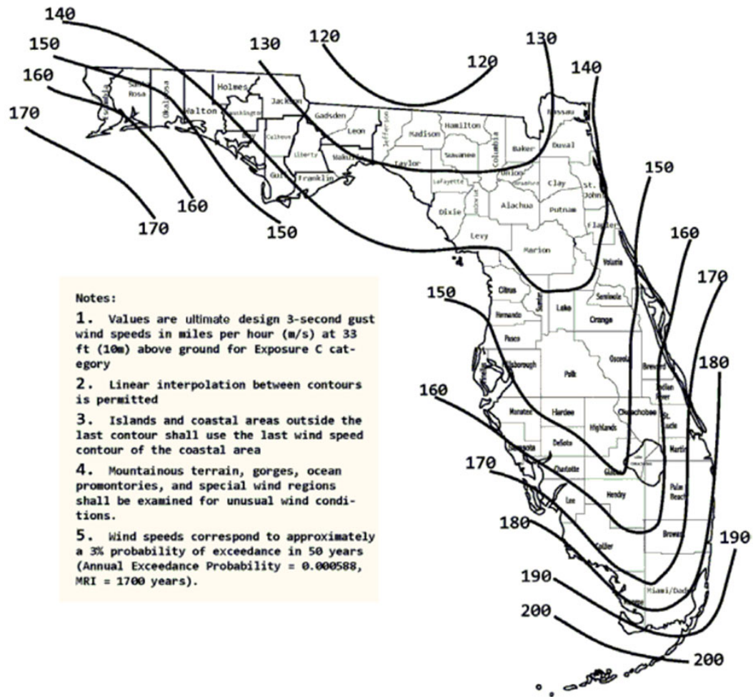
Figure A.2: Ultimate design wind speeds for Risk Category III & IV buildings and other structures (Florida Building Code, Sixth Edition Fig. 1609.3(2))
