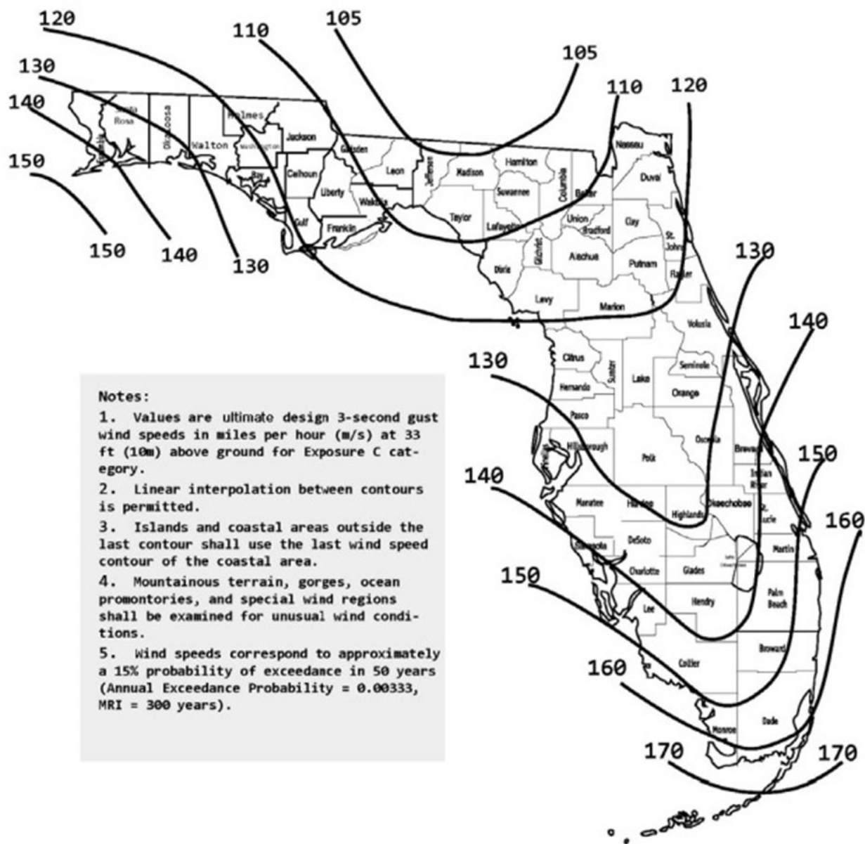
Figure A.3: Ultimate design wind speeds for Risk Category I buildings and other structures (Florida Building Code, Sixth Edition Fig. 1609.3(3))
