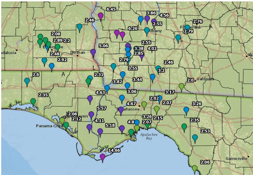
Figure 8: Reported total rainfall in the FL Panhandle resulting from Hurricane Michael (Source: National Weather Service ).
